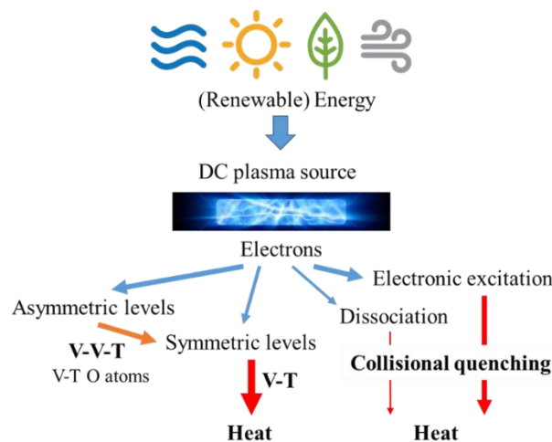
Fig. 2: Schematic overview of the flow of energy in a pure \text{CO}_2 low-pressure discharge. The red arrows stand for the main heating mechanisms involved: vibration-vibration-translation (V-V-T) relaxation, vibration-translation (V-T) and deactivation by collisions with oxygen atoms (V-T O atoms) and collisional quenching of electronic states coming from direct excitation or electron-impact dissociation of \text{CO}_2 .
